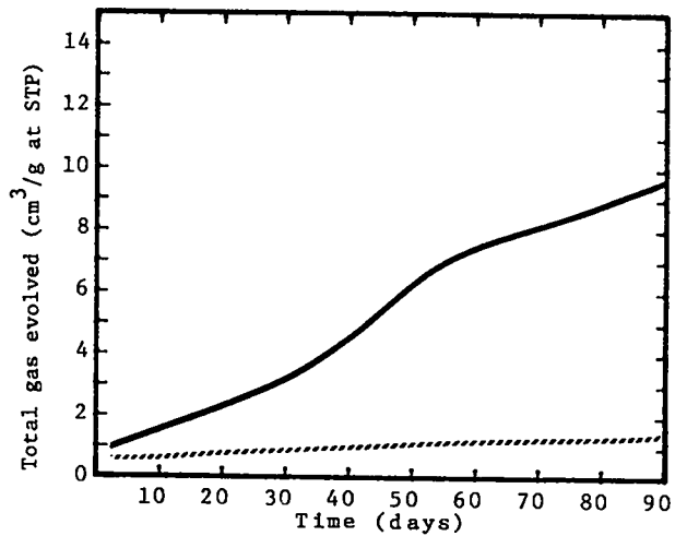
Fig. 6. DODECA (Dodecanitroquaterphenyl)
