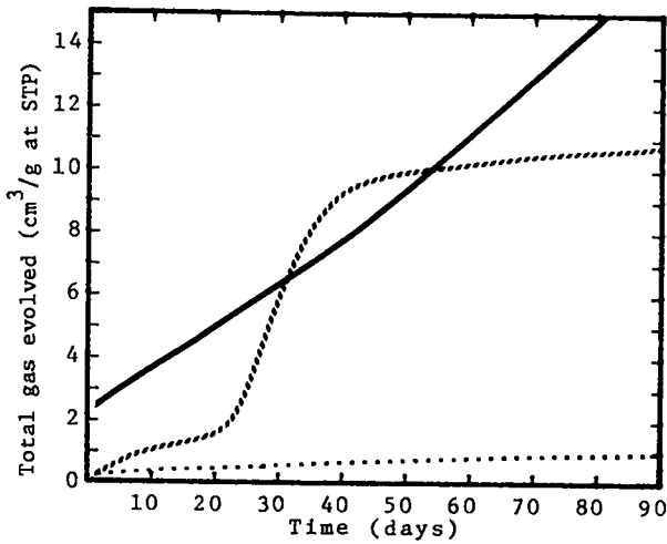
Fig. 5. DIPAM (Dipicramide)
