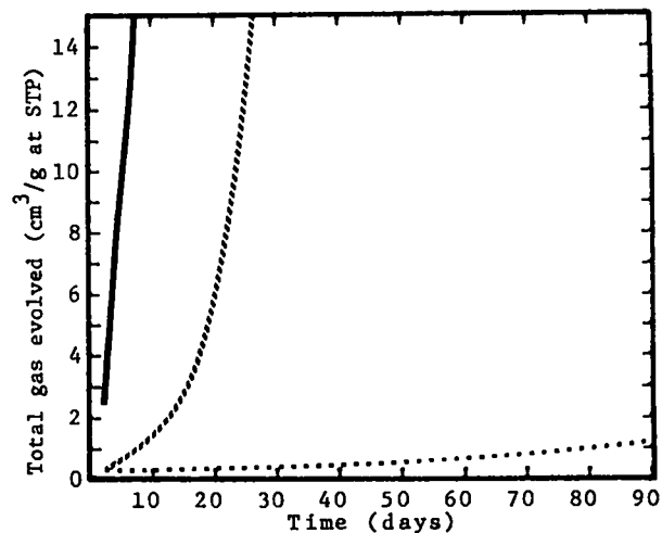
Fig. 12. HNDS (Hexanitrodiphenylsulfone)
