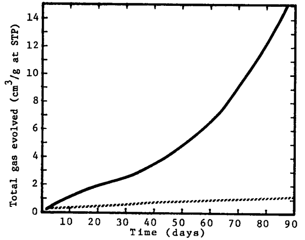
Fig. 2. BTX (Dinitropicrylbenzotriazole)
