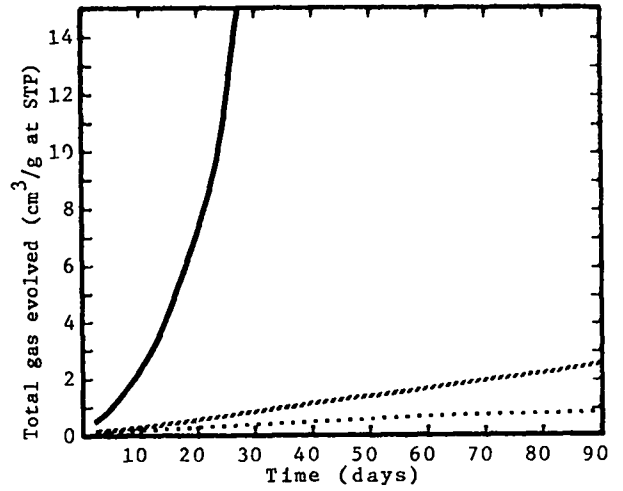
Fig. 14. KHND (Potassium salt of hexanitro-diphenylamine)
