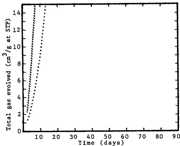
Fig. 9. HMX (Octahydro-tetra-nitro-s-tetrazine)
