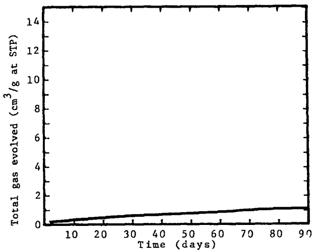
Fig. 27. TPT (Tripicryltriiazine)
