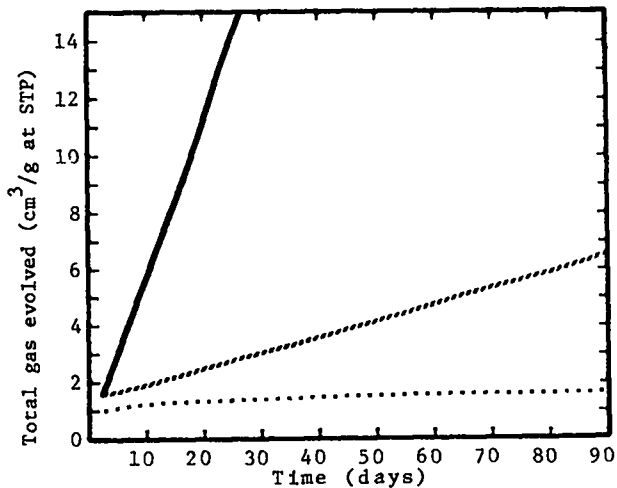
Fig. 26. TPM (Tripicrylmelamine)
