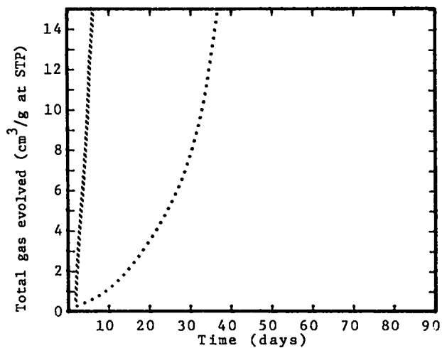
Fig. 21. RDX (Hexahydrotrinitro-s-triazine)
