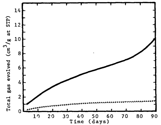
Fig. 18. PATO (Picrylamino-triazole)
