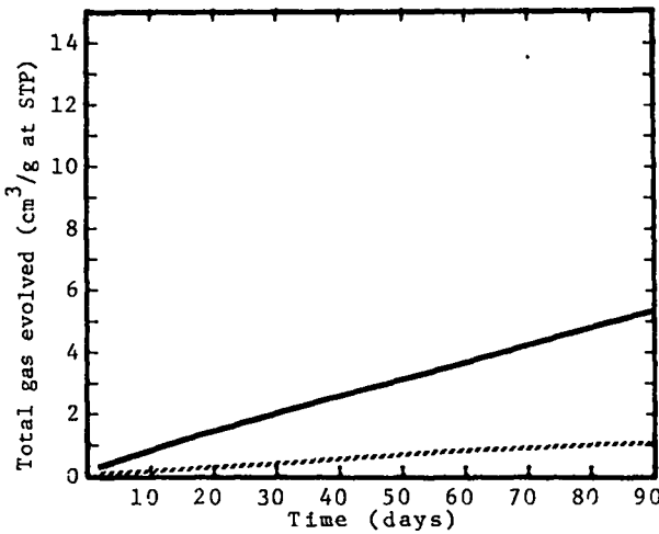
Fig. 15. NONA (Nonanitroterphenyl)
