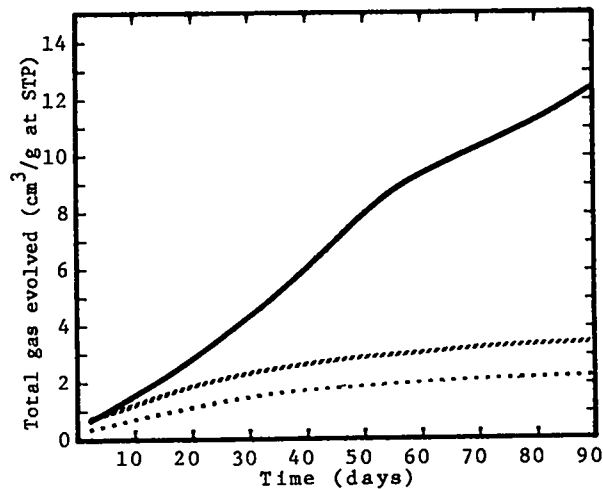
Fig. 8. DPPM (Dipicrylpyromellitide)
