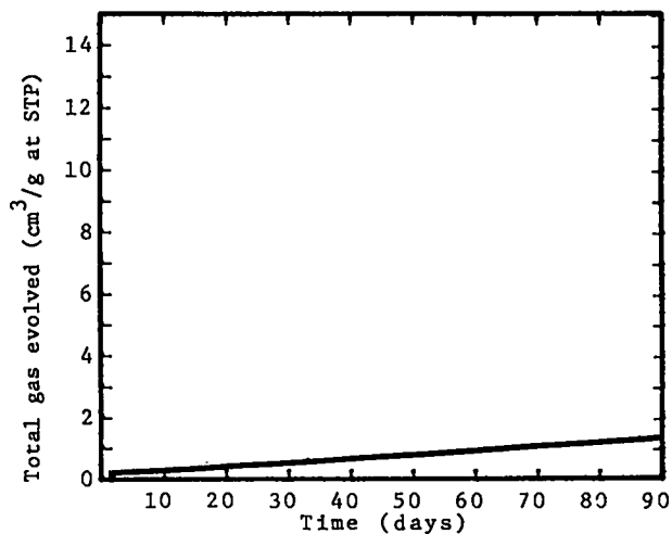
Fig. 19. Penco (Pentanitrobenzophenone)
