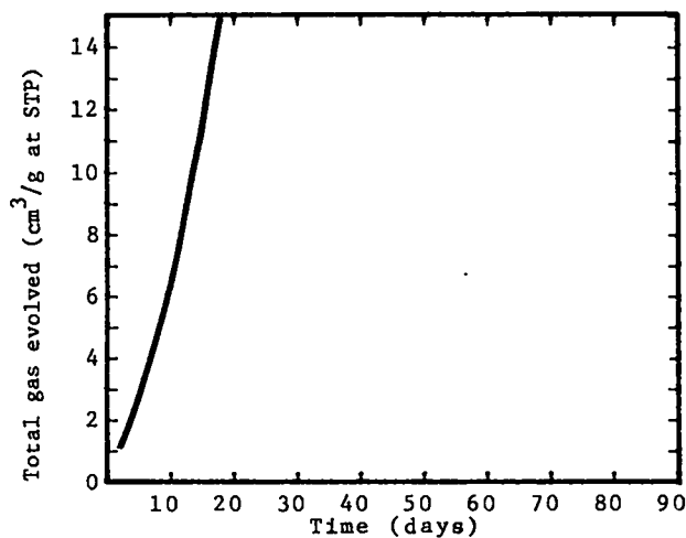
Fig. 23. TATB (Triaminotrinitrobenzene) Recrystallized from DMSO
